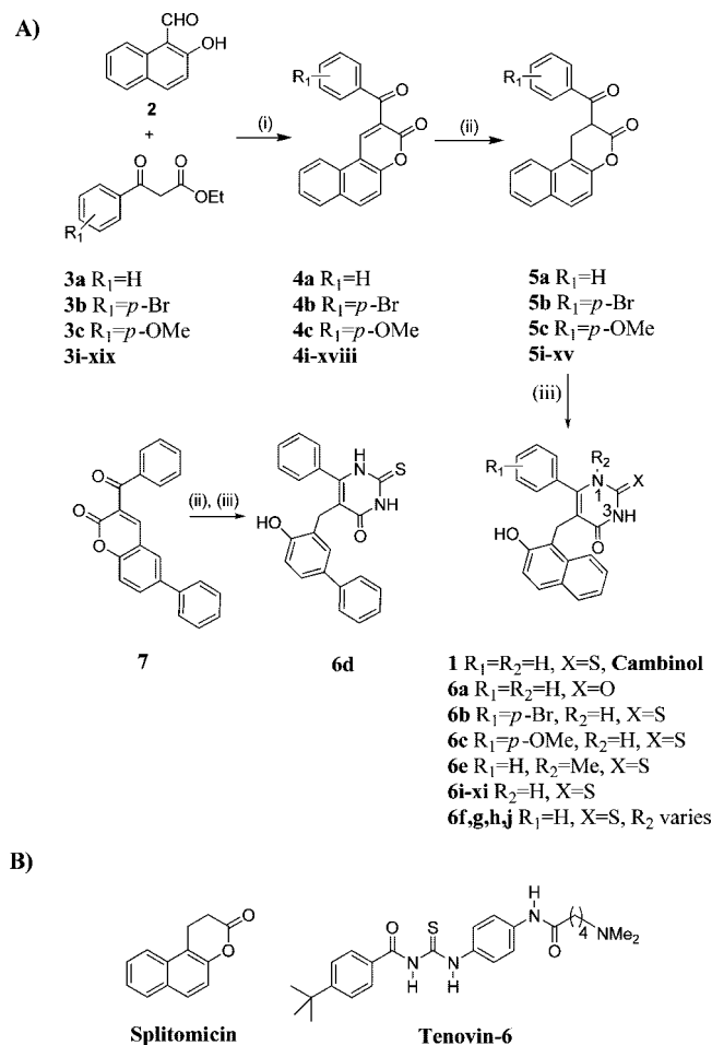
Scheme 1. (A) Synthesis of 1 and 6a–j a and (B) Structural Comparison of Tenovin-6 and Splitomicin
